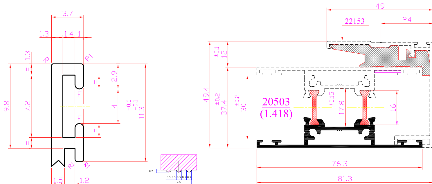
DETAIL-I GULF EXTRUSIONS (IDENTIFICATION MARK)
