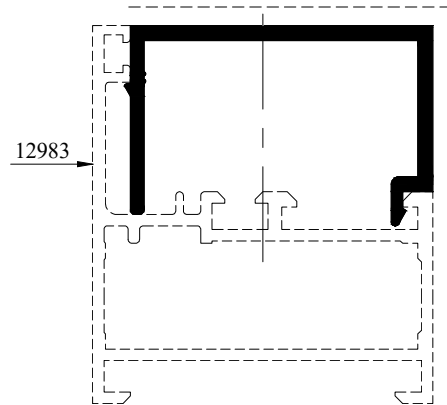
DETAIL-I GULF EXTRUSIONS (IDENTIFICATION MARK)
