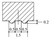
DETAIL-I GULF EXTRUSIONS (IDENTIFICATION MARK)
