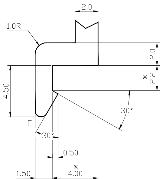
DETAIL-X
